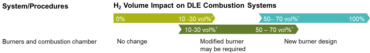
Figure 7: Hydrogen fuel volume impacts on DLE combustion systems
