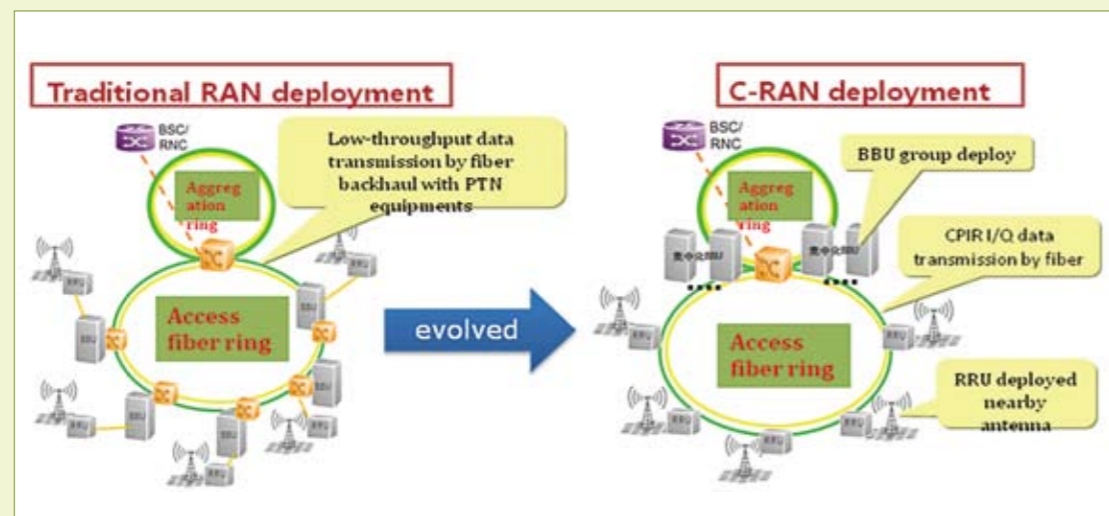
Figure 3 Typical C-RAN Deployment Topology vs. Traditional RAN Mode
