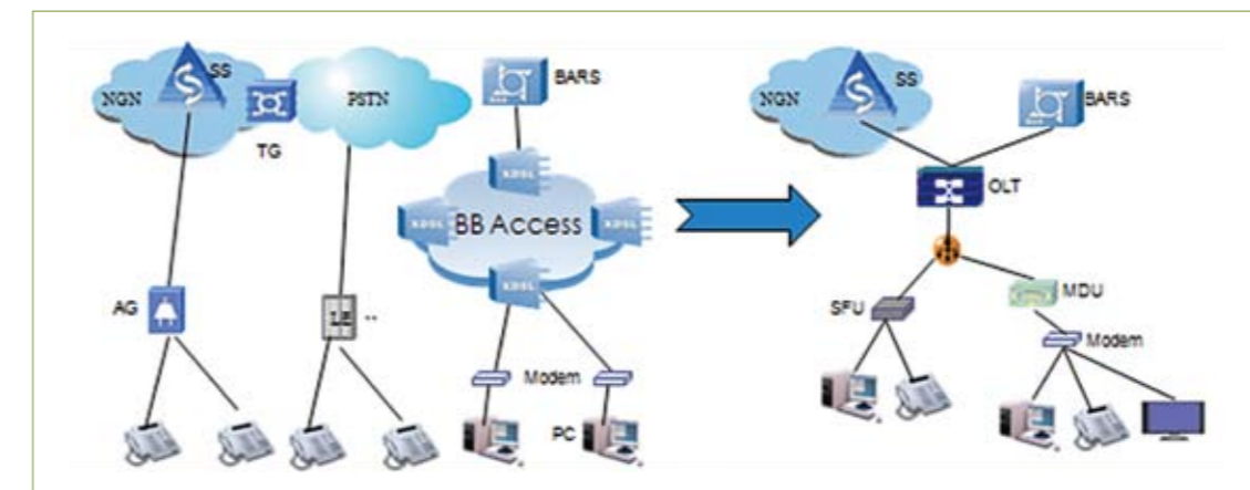
Figure 4 FTTx Network to make Multi Access Network Convergence
