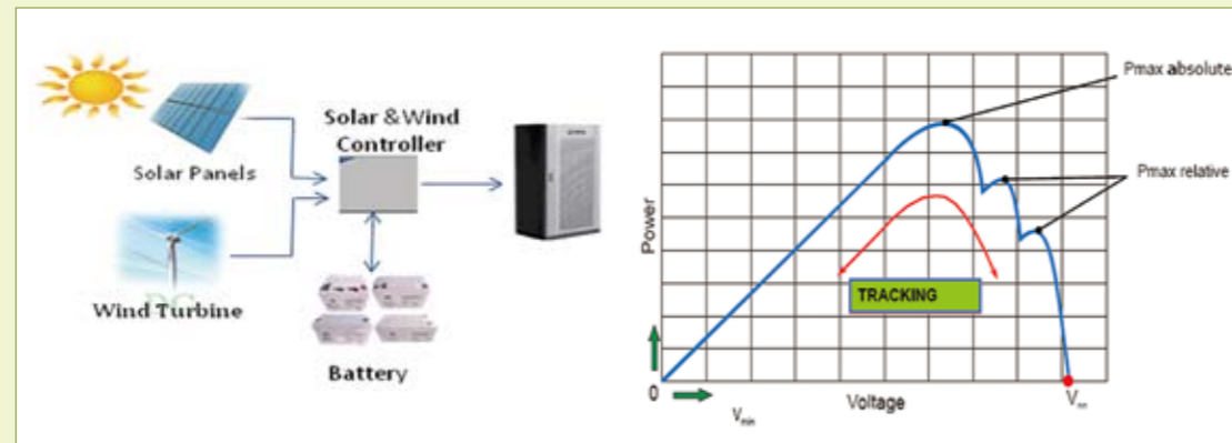
Figure 9 Hybrid wind and solar system with MPPT controller state
