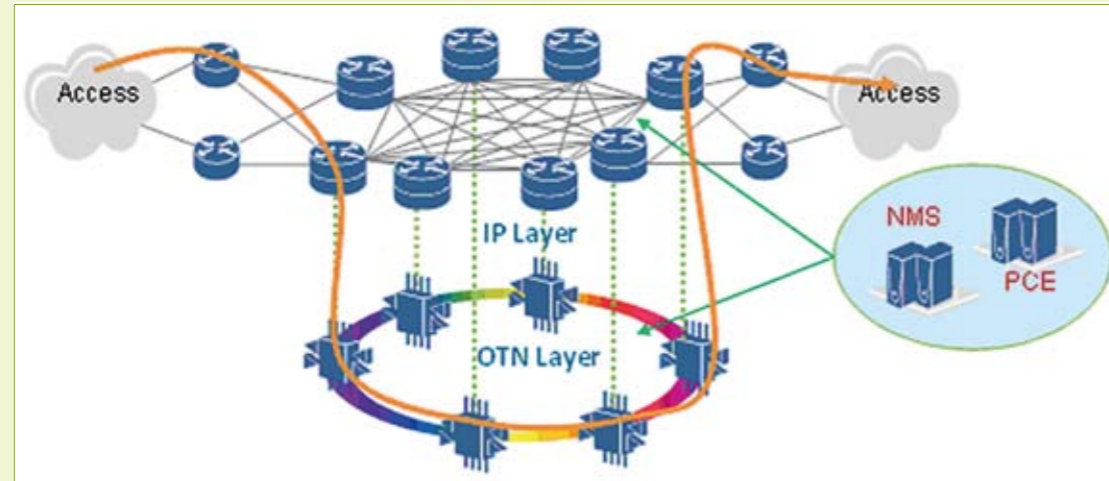
Figure 6 Integrated-bearer solution for IP layer and OTN layer
