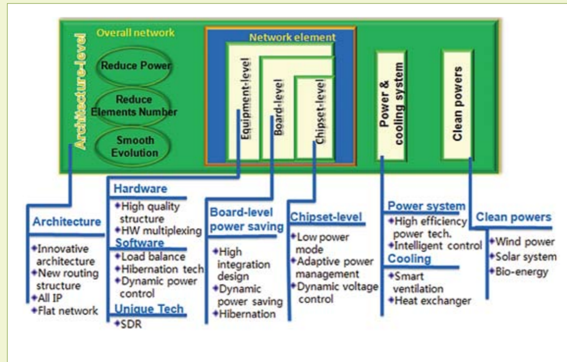
Figure 1 Overall analysis of power saving technologies
